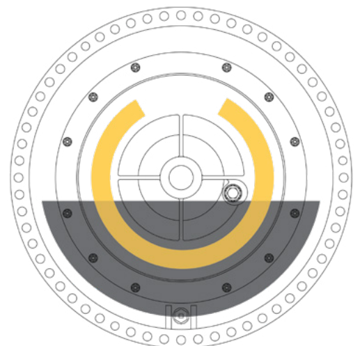
The Birrana™ oil sampling plug can take samples anywhere between 30° and 330°
